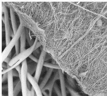
RIFTELEN® N15 cross-section
